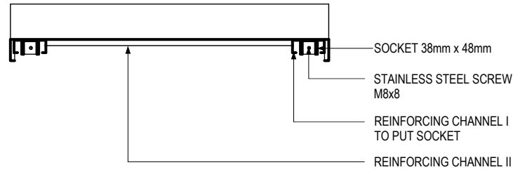
A-SECTION VIEW SCALE 1:15mm
